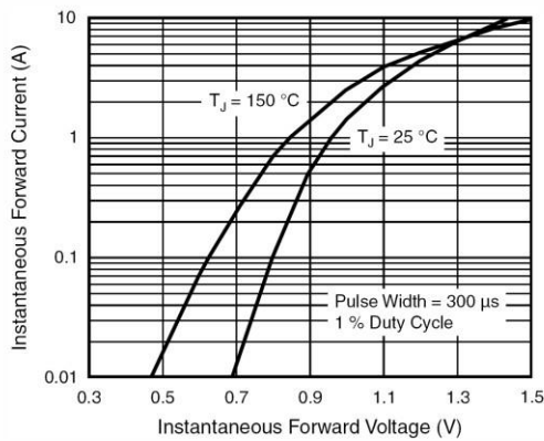
Figure 3. Typical Forward Voltage Characteristics Per Diode
